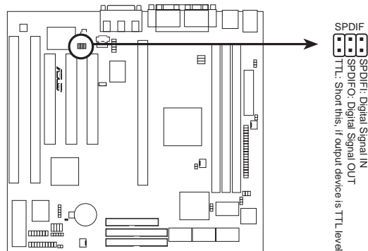
P2L-VM/P2E-VM Digital Audio Interface
